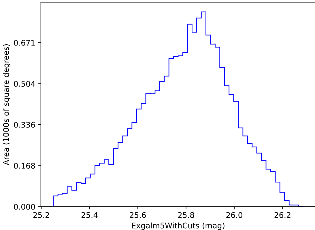
weather_cloudso31v3.4_10yrs i band non-DD year 3: ExgalM5WithCuts
