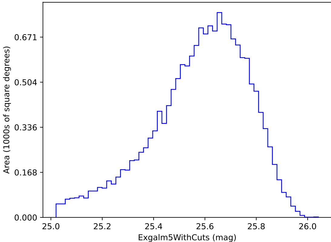
weather_cloudso31v3.4_10yrs i band non-DD year 2: ExgalM5WithCuts
