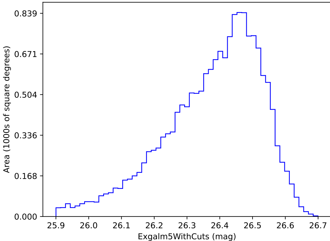
weather_cloudso31v3.4_10yrs i band non-DD year 10: Exgalml5WithCuts
