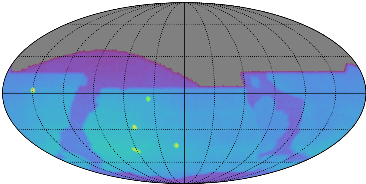
weather_cloudso31v3.4_10yrs : Brown Dwarf, L4
