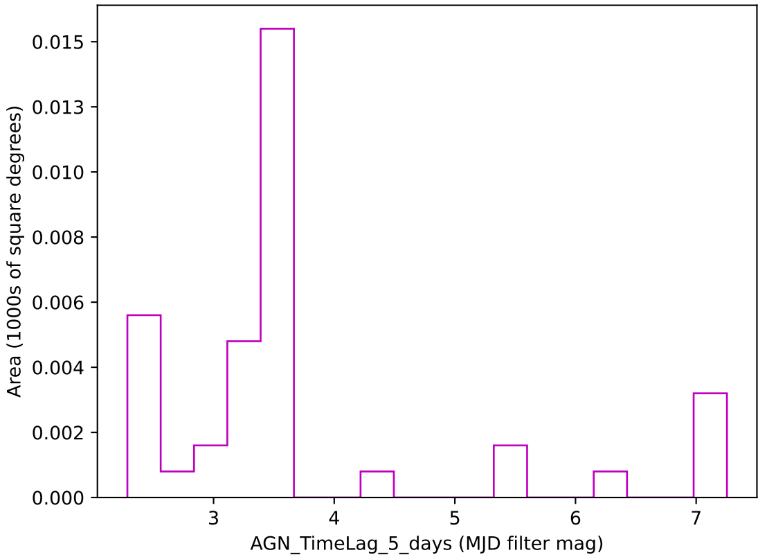
weather_cloudso31v3.4_10yrs z band: AGN_TimeLag_5_days
