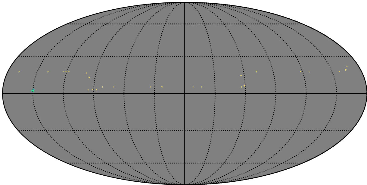
weather_cloudso31v3.4_10yrs y band: AGN_TimeLag_5_days
