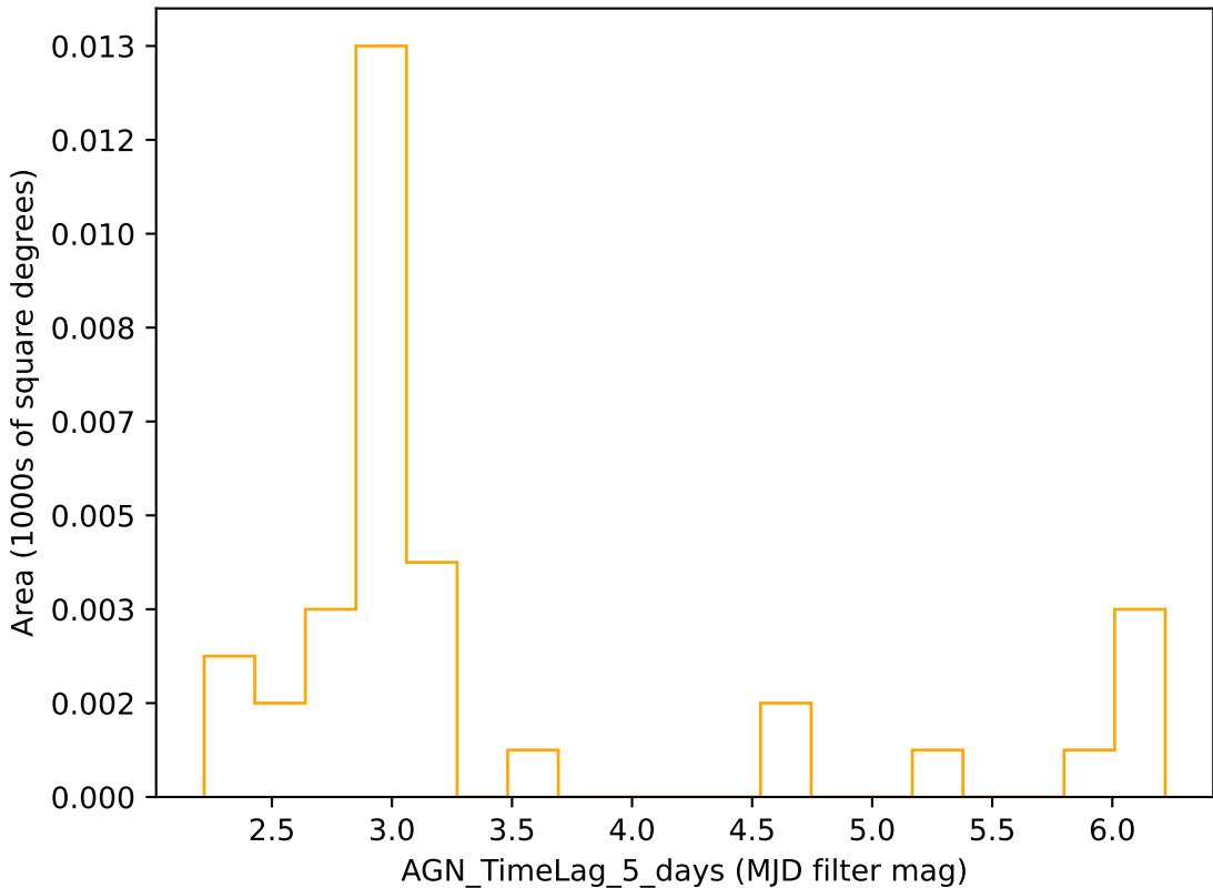
weather_cloudso31v3.4_10yrs r band: AGN_TimeLag_5_days
