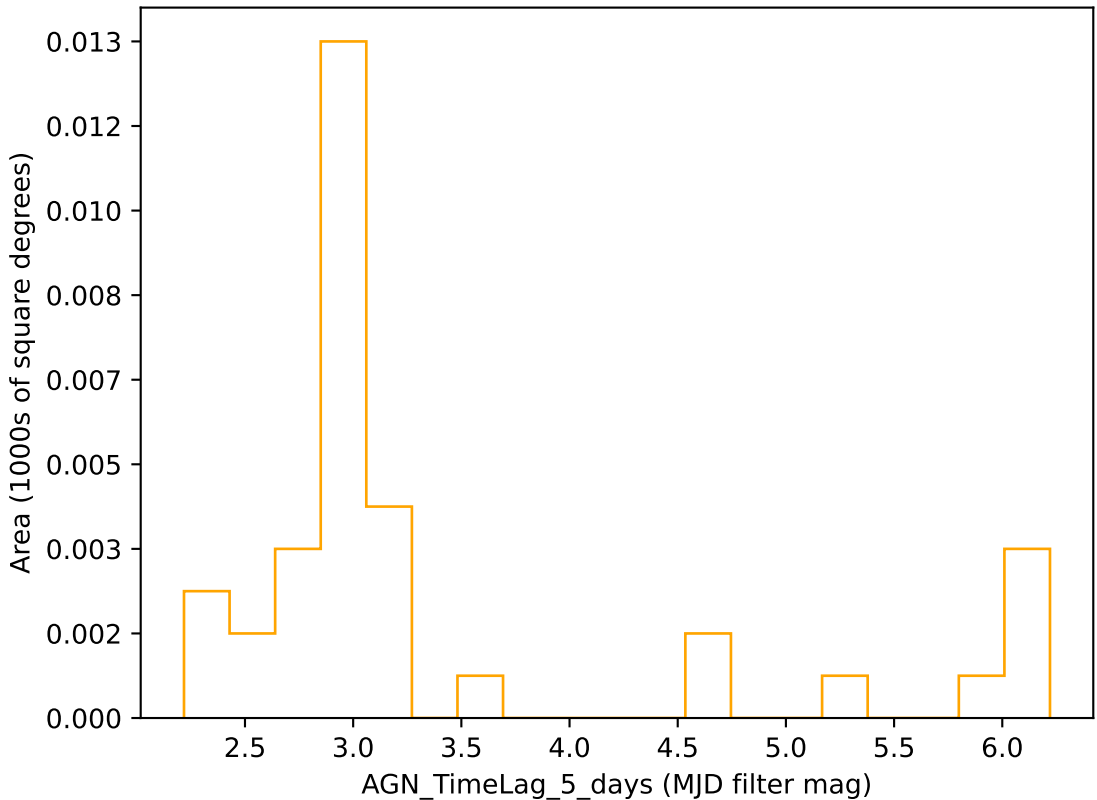
weather_cloudso31v3.4_10yrs r band: AGN_TimeLag_5_days
