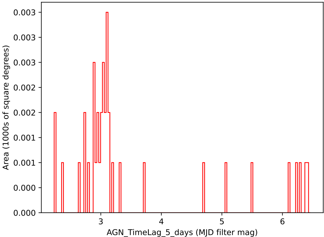
weather_cloudso31v3.4_10yrs i band: AGN_TimeLag_5_days
