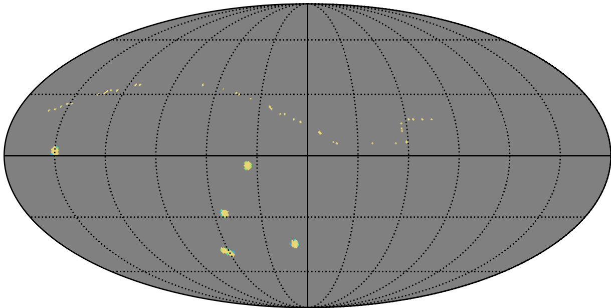
weather_cloudso31v3.4_10yrs all bands: AGN_TimeLag_5_days
