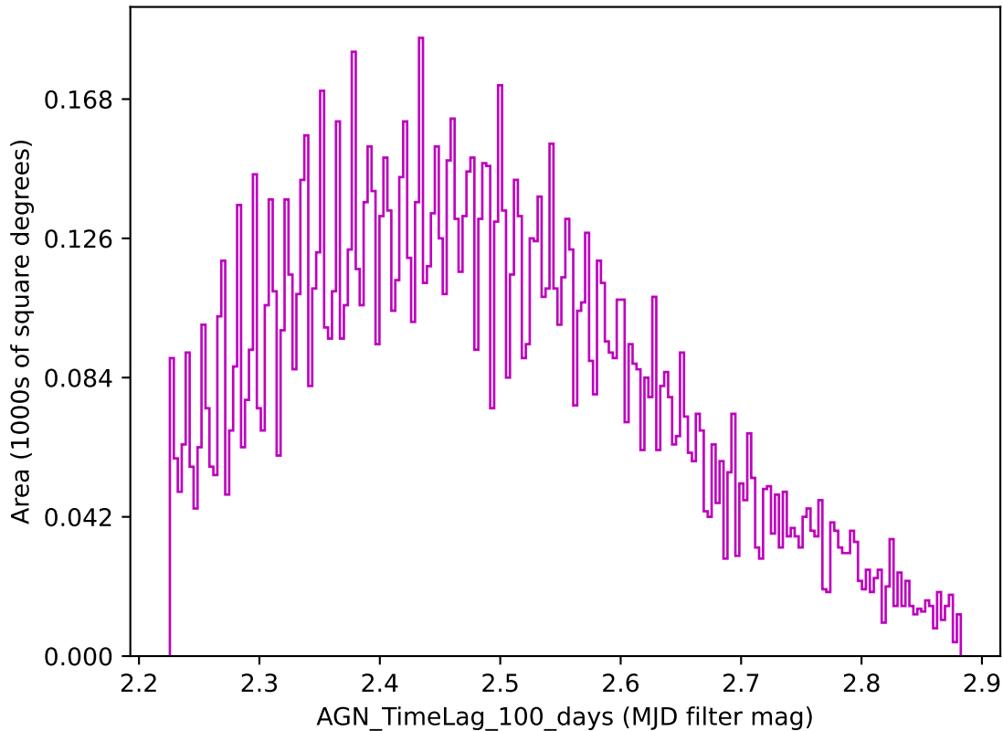
weather_cloudso31v3.4_10yrs z band: AGN_TimeLag_100_days
