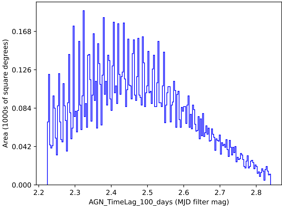
weather_cloudso31v3.4_10yrs y band: AGN_TimeLag_100_days
