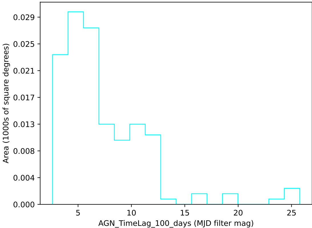
weather_cloudso31v3.4_10yrs u band: AGN_TimeLag_100_days
