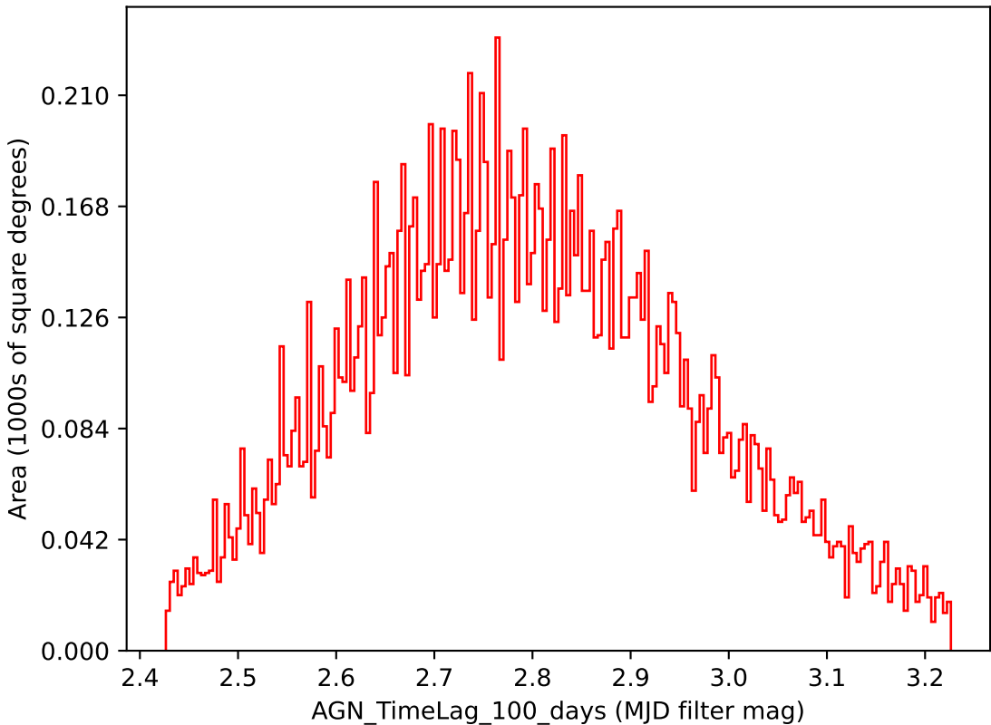
weather_cloudso31v3.4_10yrs i band: AGN_TimeLag_100_days
