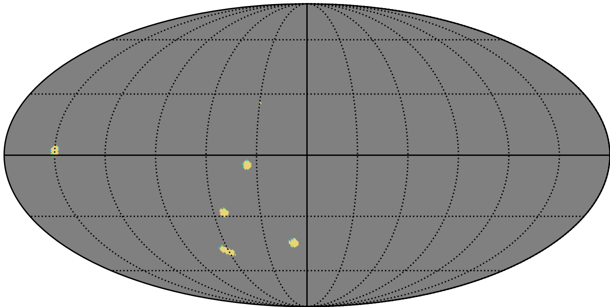
weather_cloudso31v3.4_10yrs g band: AGN_TimeLag_100_days
