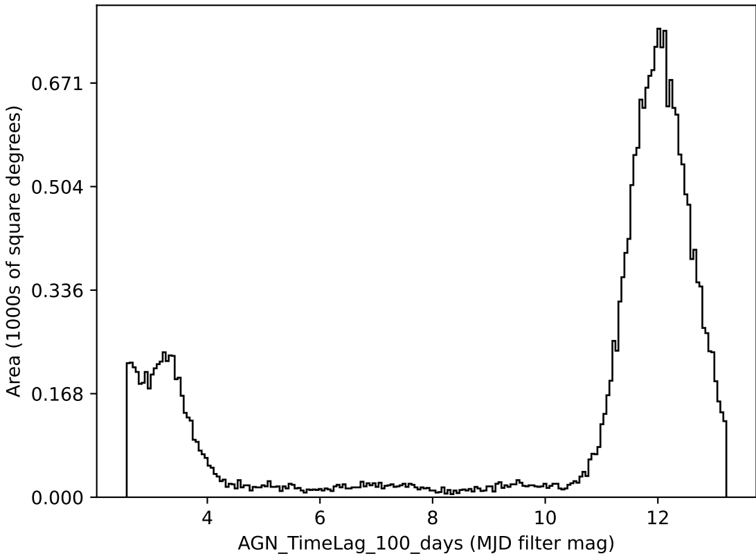
weather_cloudso31v3.4_10yrs all bands: AGN_TimeLag_100_days
