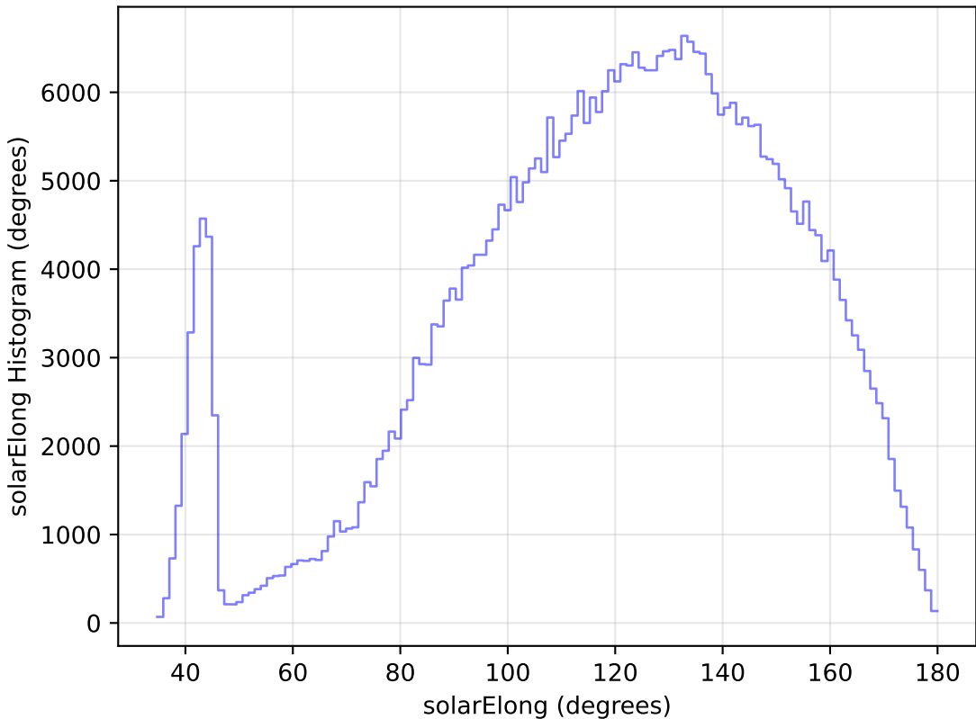
weather_cloudso31v3.4_10yrs WFD z band: solarElong Histogram
