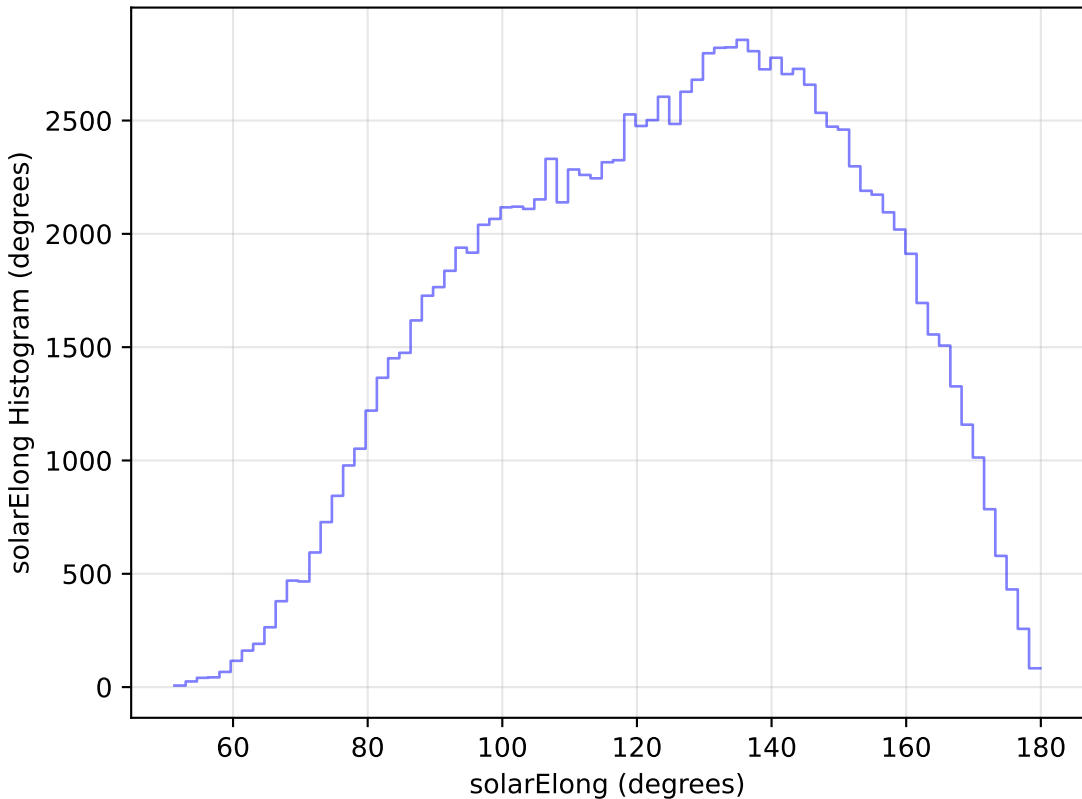
weather_cloudso31v3.4_10yrs WFD u band: solarElong Histogram
