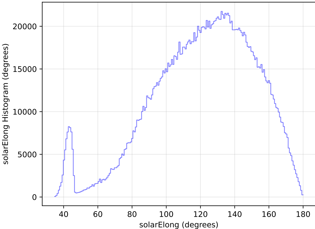
weather_cloudso31v3.4_10yrs WFD all bands: solarElong Histogram
