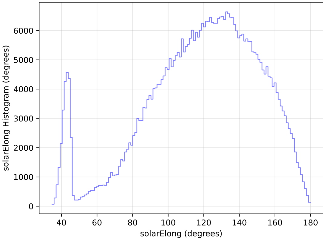
weather_cloudso31v3.4_10yrs All sky z band: solarElong Histogram
