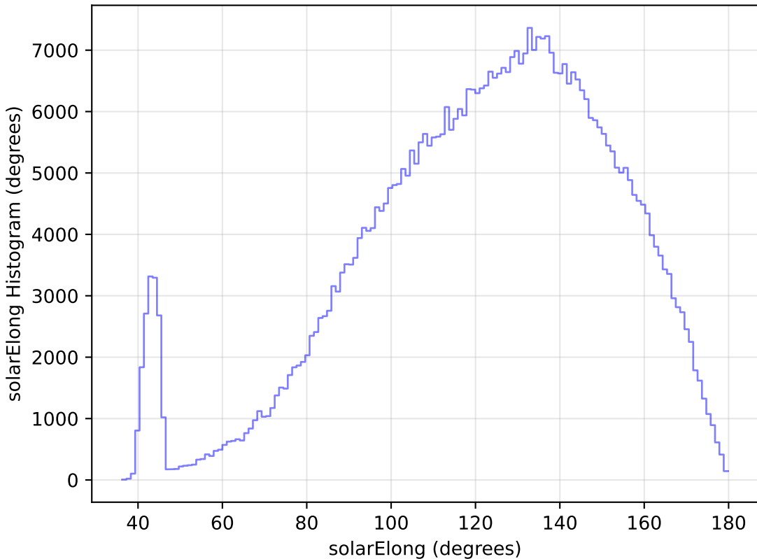
weather_cloudso31v3.4_10yrs All sky r band: solarElong Histogram
