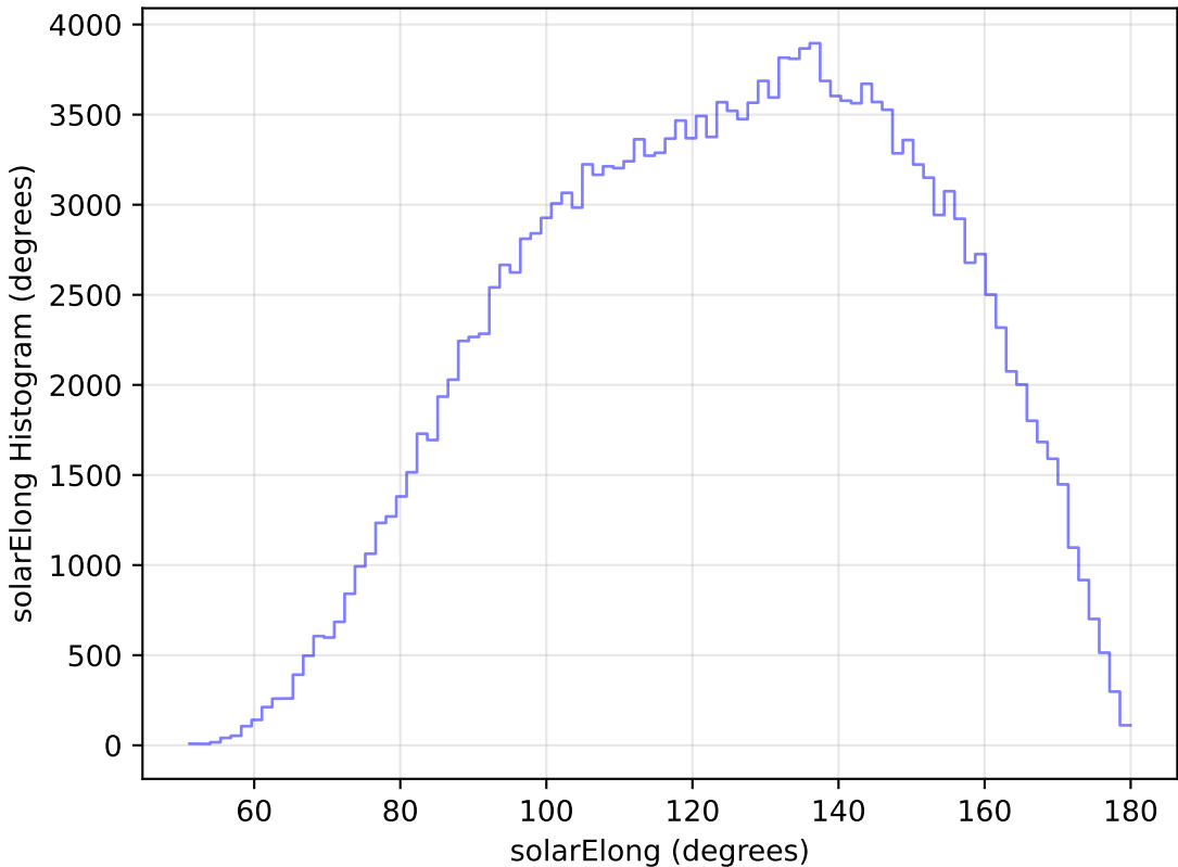
weather_cloudso31v3.4_10yrs All sky g band: solarElong Histogram
