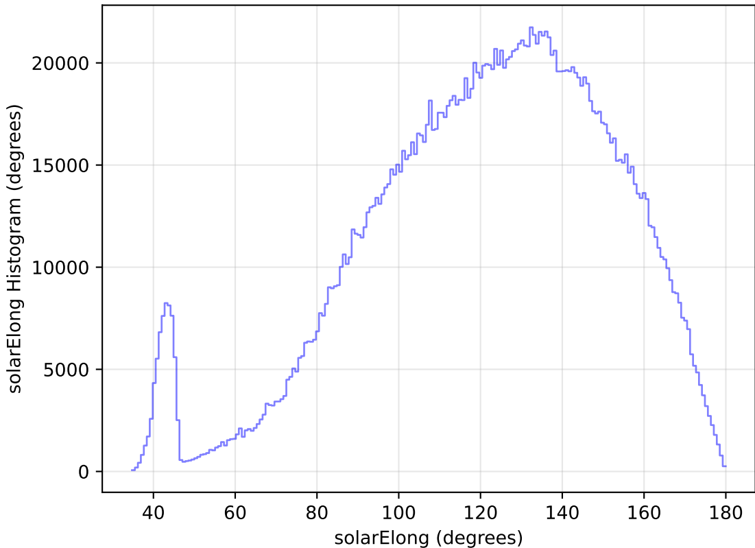
weather_cloudso31v3.4_10yrs All sky all bands: solarElong Histogram
