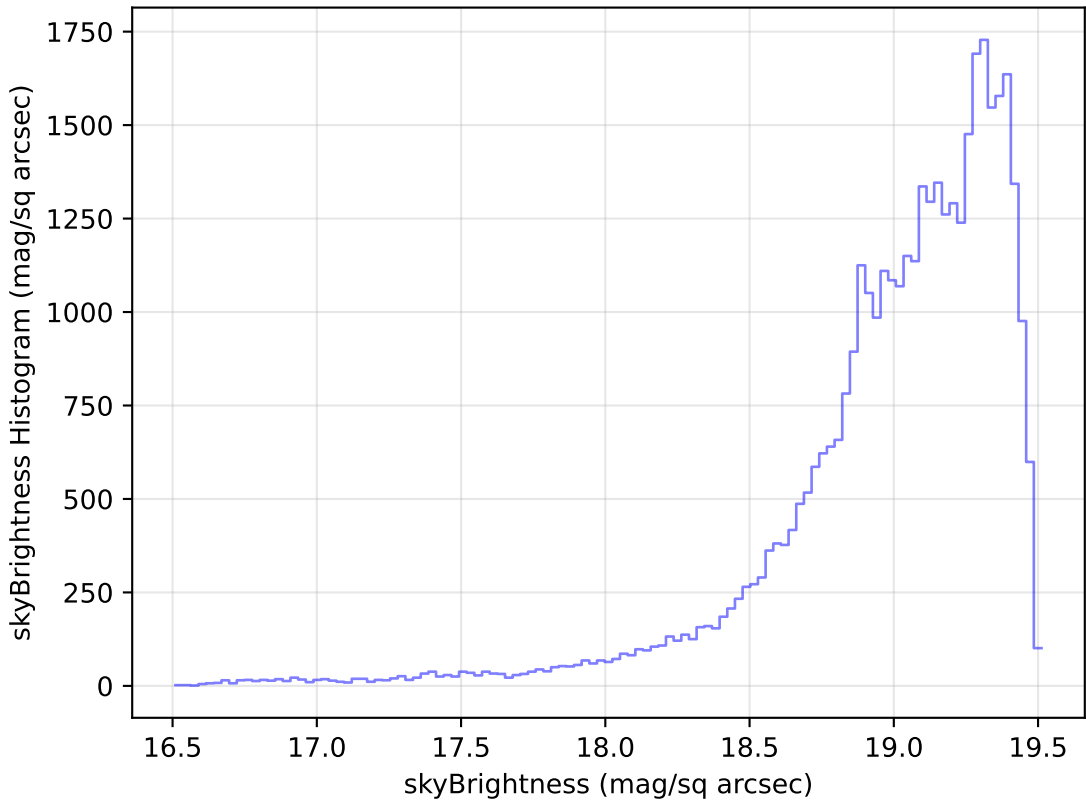
weather_cloudso31v3.4_10yrs Yr 1 z band: skyBrightness Histogram
