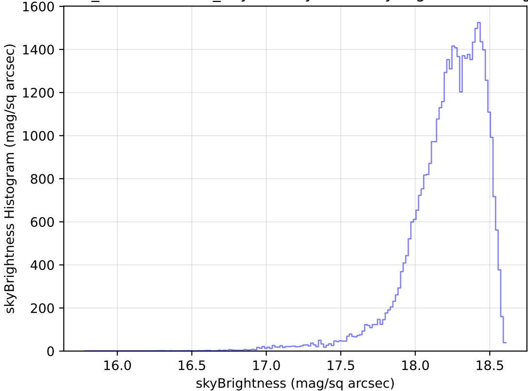
weather_cloudso31v3.4_10yrs Yr 1 y band: skyBrightness Histogram
