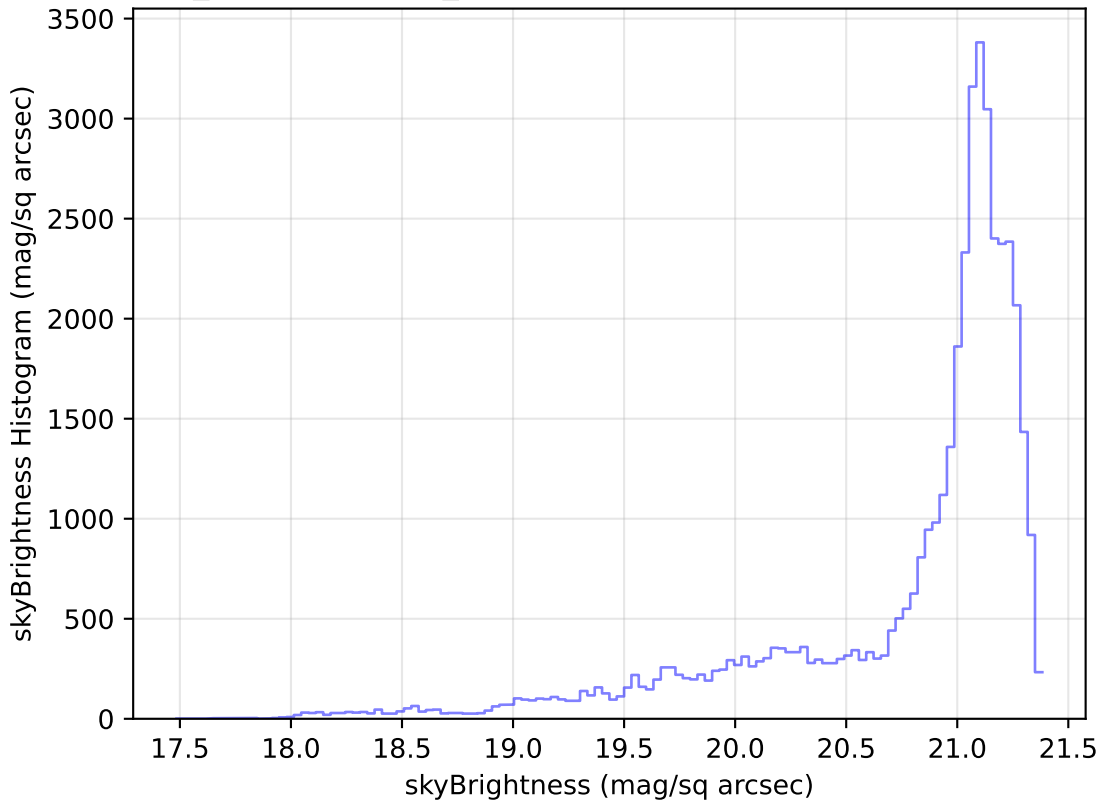
weather_cloudso31v3.4_10yrs Yr 1 r band: skyBrightness Histogram
