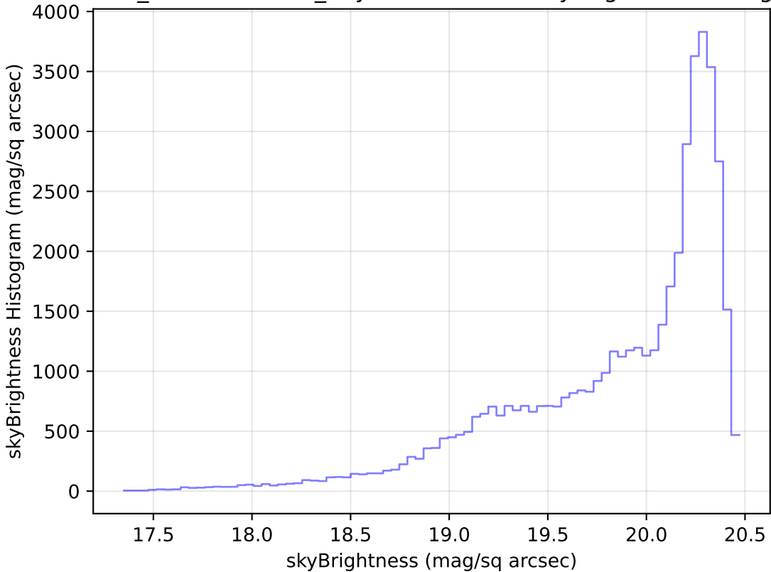
weather_cloudso31v3.4_10yrs Yr 1 i band: skyBrightness Histogram
