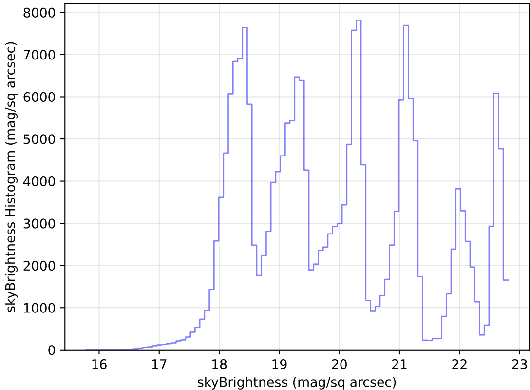
weather_cloudso31v3.4_10yrs Yr 1 all bands: skyBrightness Histogram
