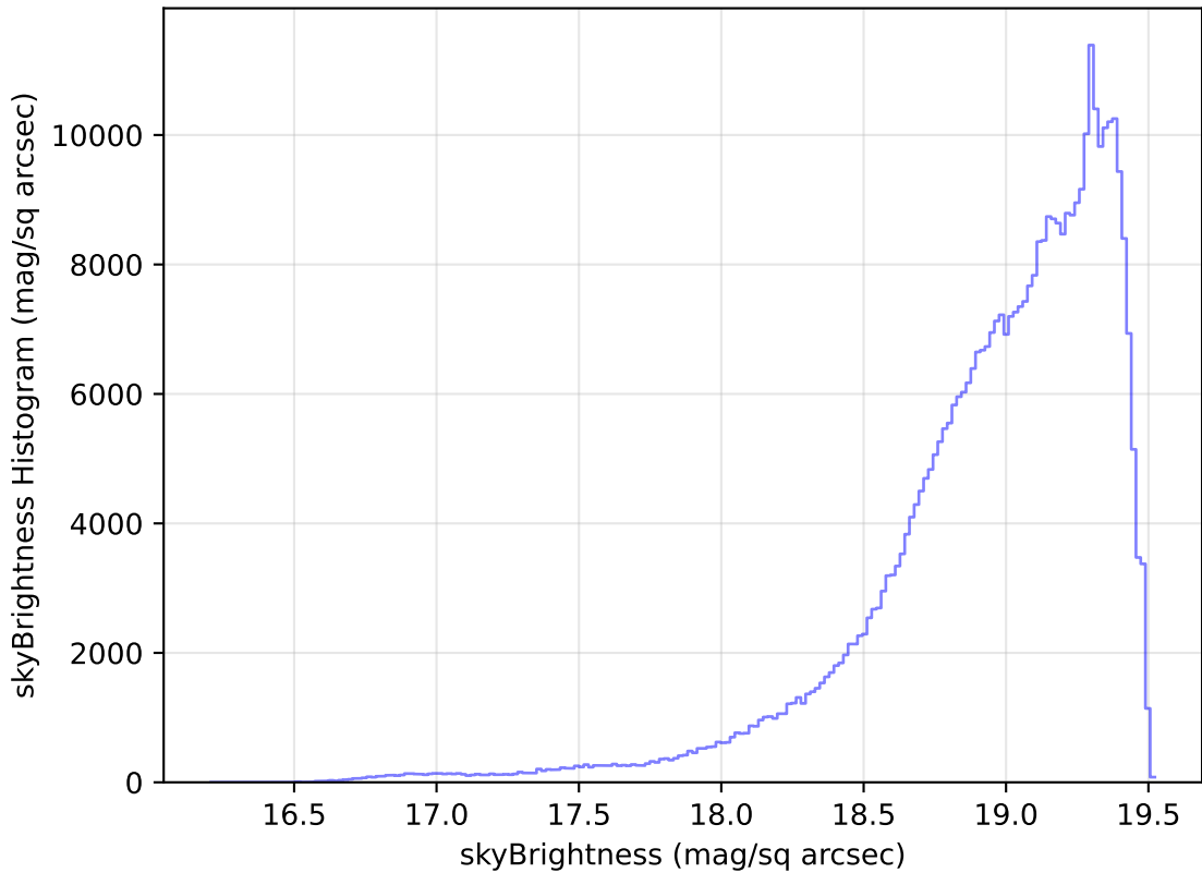
weather_cloudso31v3.4_10yrs WFD z band: skyBrightness Histogram
