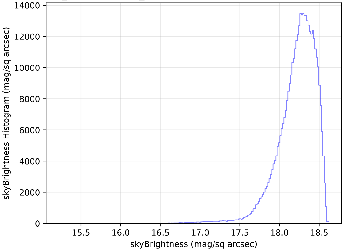
weather_cloudso31v3.4_10yrs WFD y band: skyBrightness Histogram
