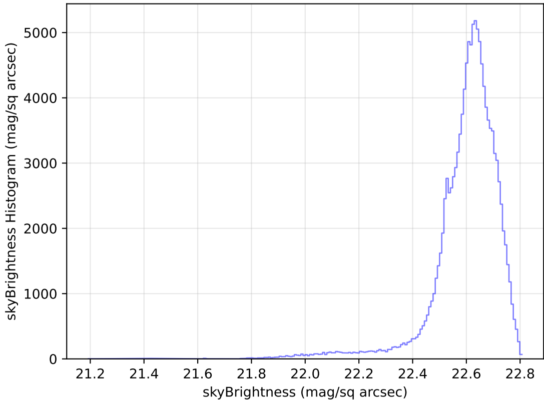
weather_cloudso31v3.4_10yrs WFD u band: skyBrightness Histogram
