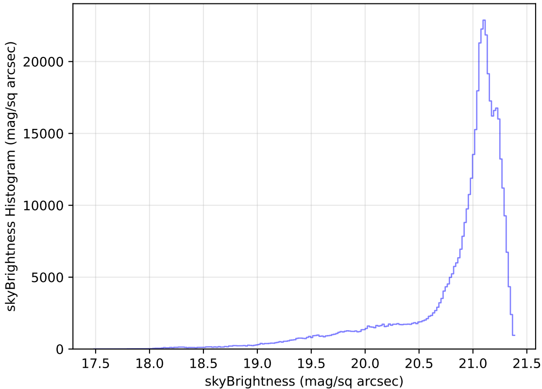
weather_cloudso31v3.4_10yrs WFD r band: skyBrightness Histogram
