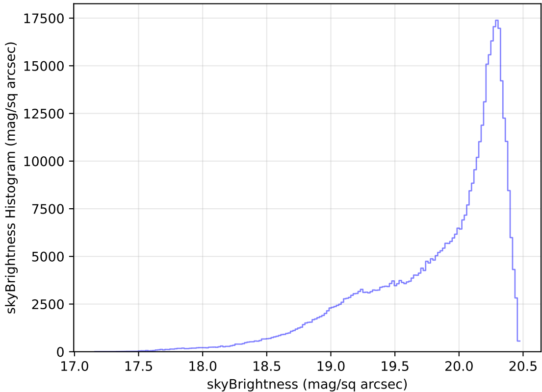
weather_cloudso31v3.4_10yrs WFD i band: skyBrightness Histogram
