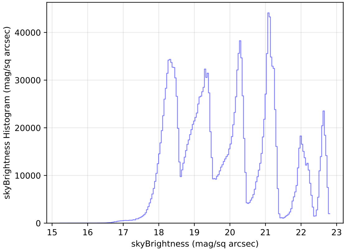
weather_cloudso31v3.4_10yrs WFD all bands: skyBrightness Histogram
