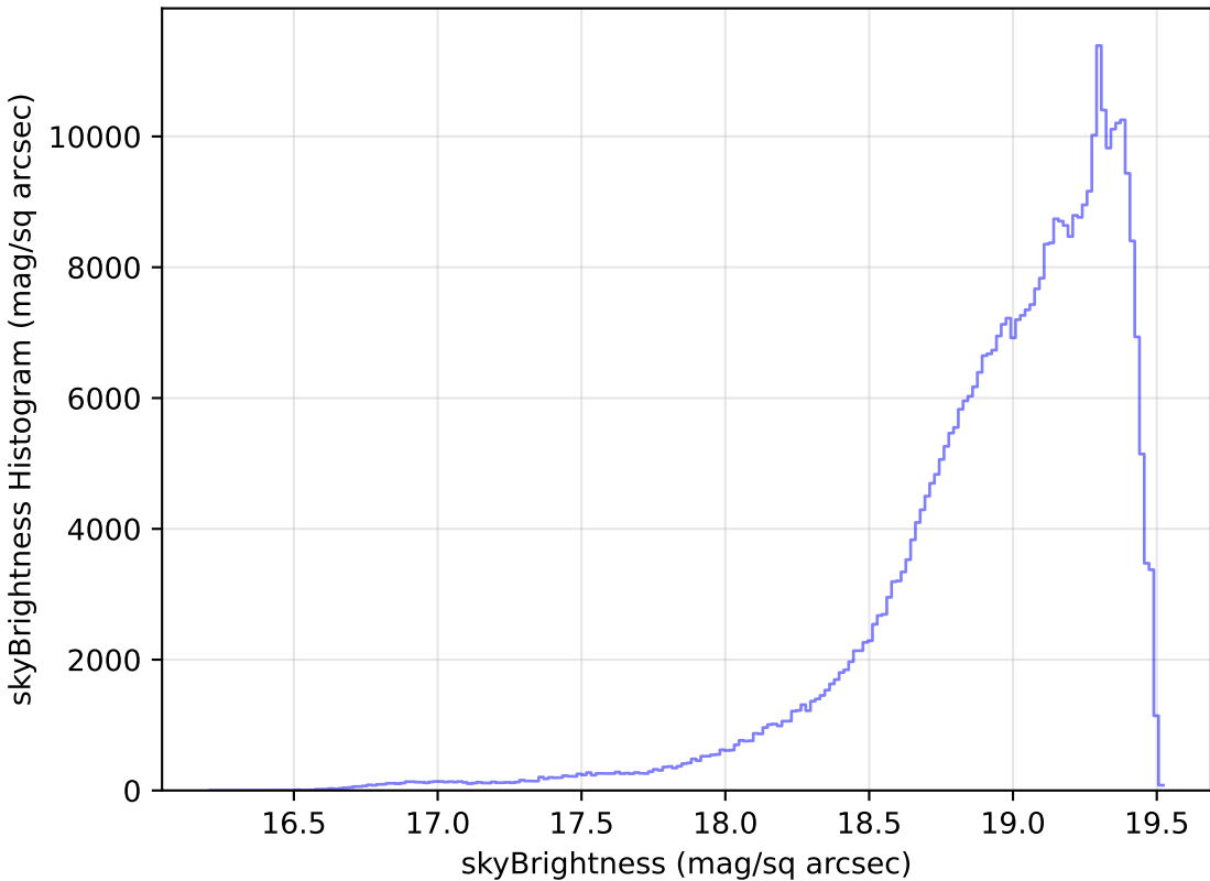
weather_cloudso31v3.4_10yrs All sky z band: skyBrightness Histogram
