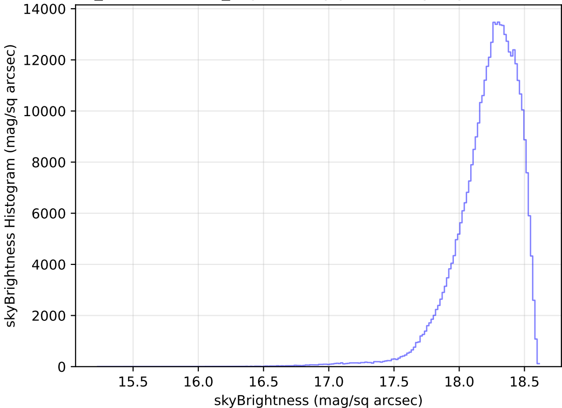
weather_cloudso31v3.4_10yrs All sky y band: skyBrightness Histogram
