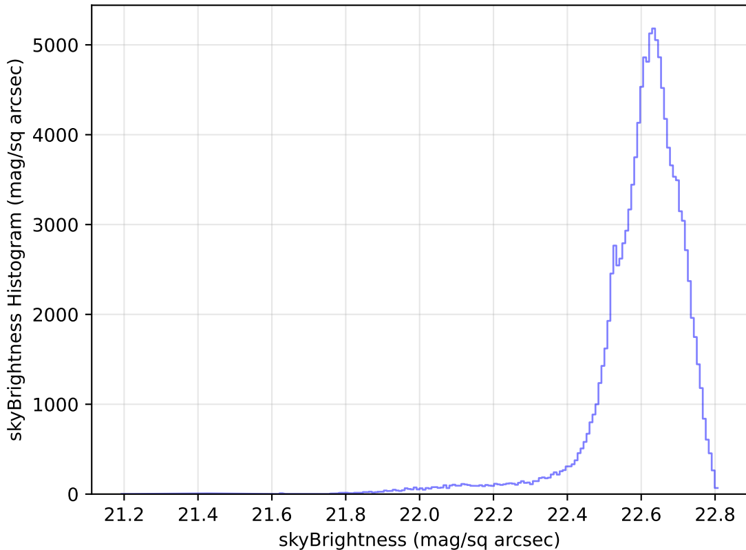
weather_cloudso31v3.4_10yrs All sky u band: skyBrightness Histogram
