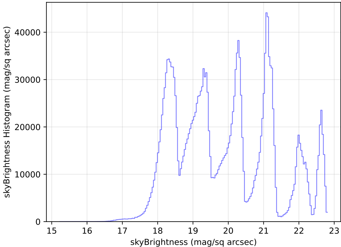
weather_cloudso31v3.4_10yrs All sky all bands: skyBrightness Histogram
