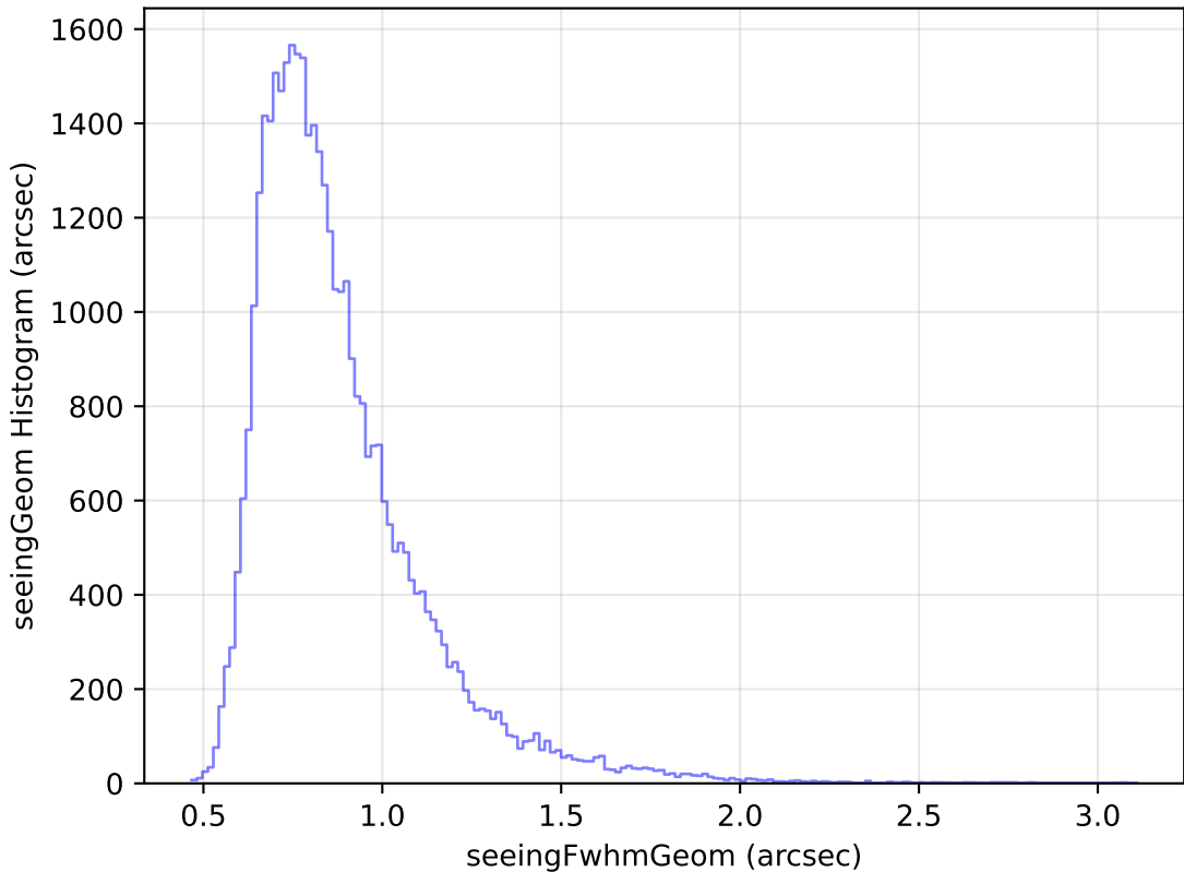
weather_cloudso31v3.4_10yrs Yr 1 z band: seeingGeom Histogram
