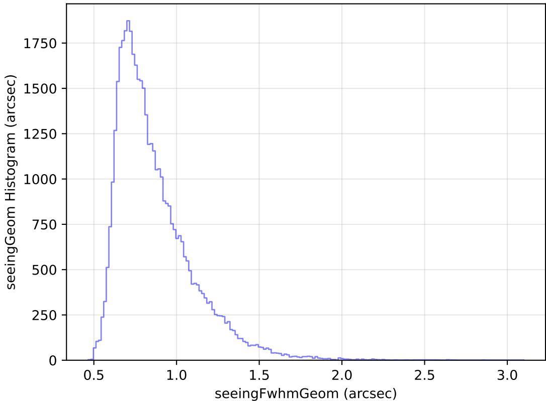
weather_cloudso31v3.4_10yrs Yr 1 r band: seeingGeom Histogram
