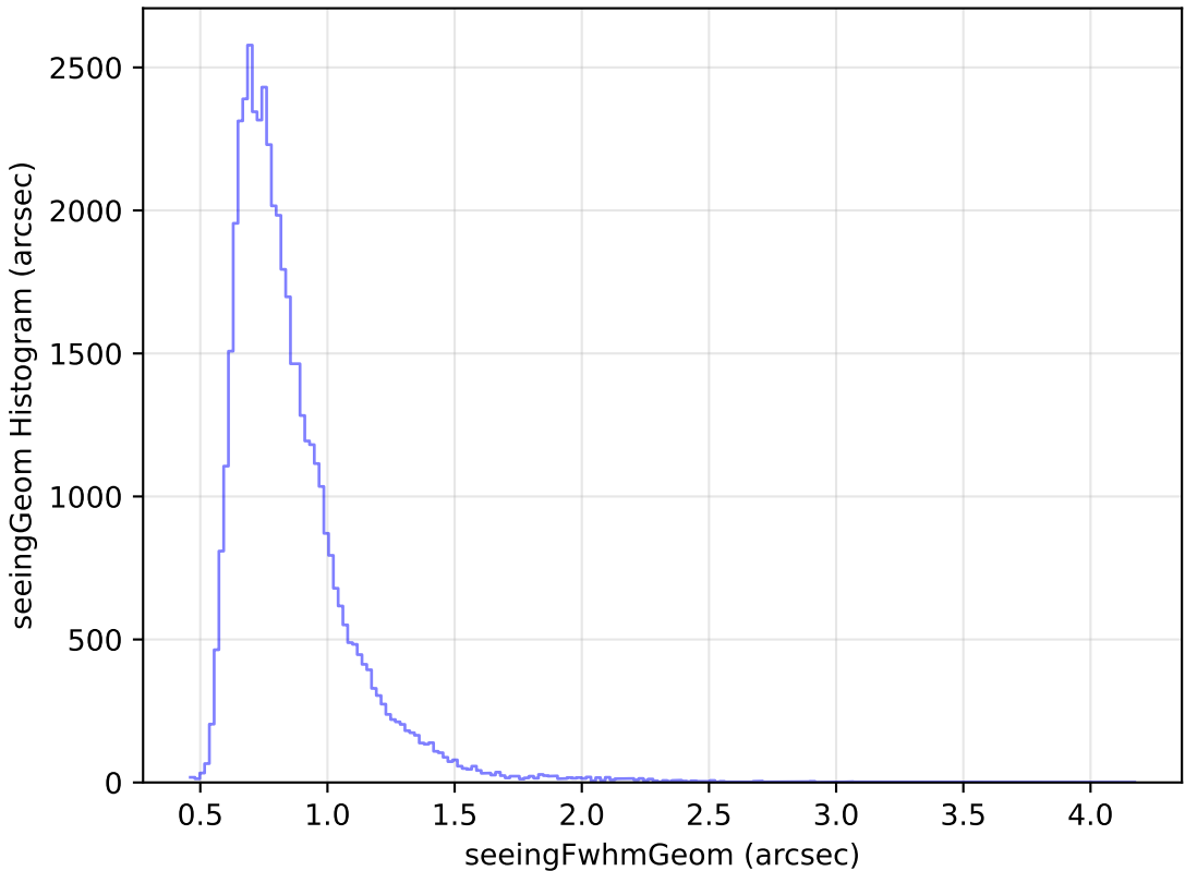
weather_cloudso31v3.4_10yrs Yr 1 i band: seeingGeom Histogram
