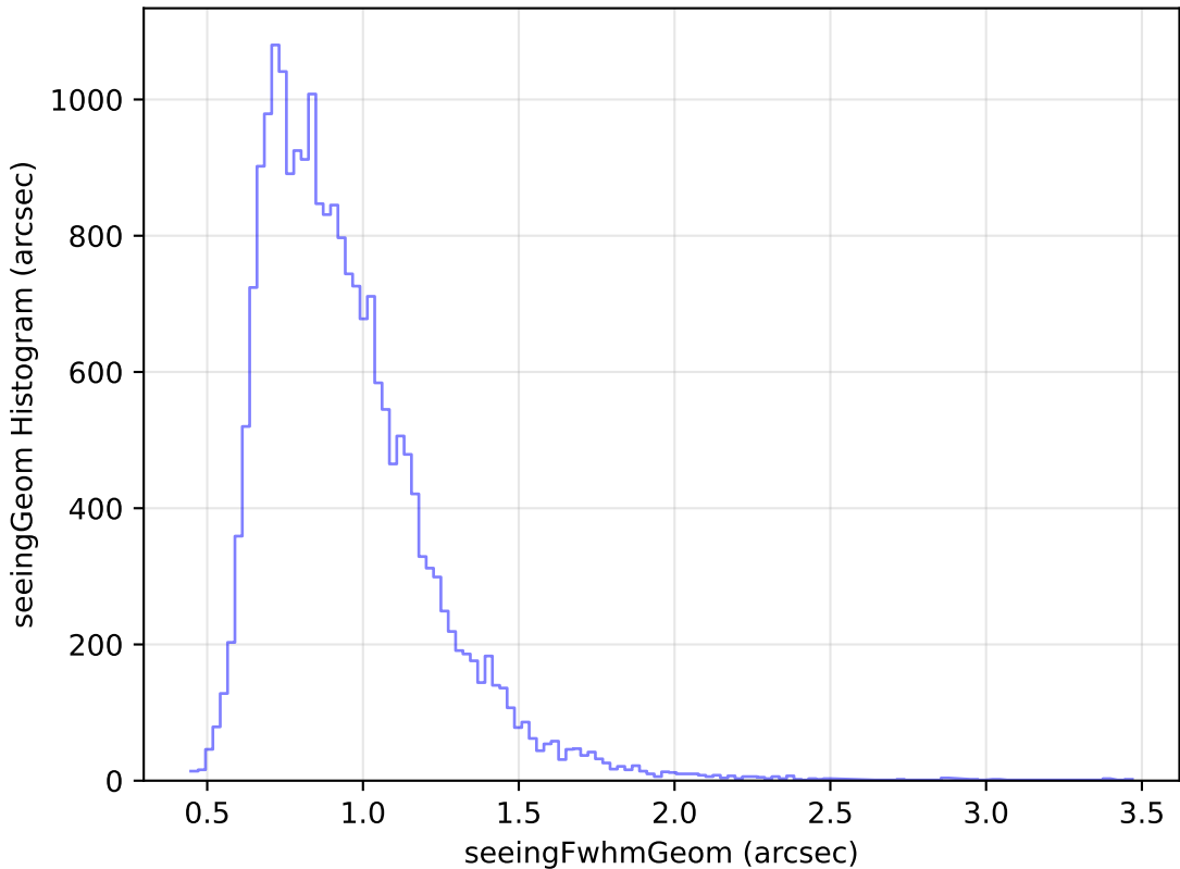
weather_cloudso31v3.4_10yrs Yr 1 g band: seeingGeom Histogram
