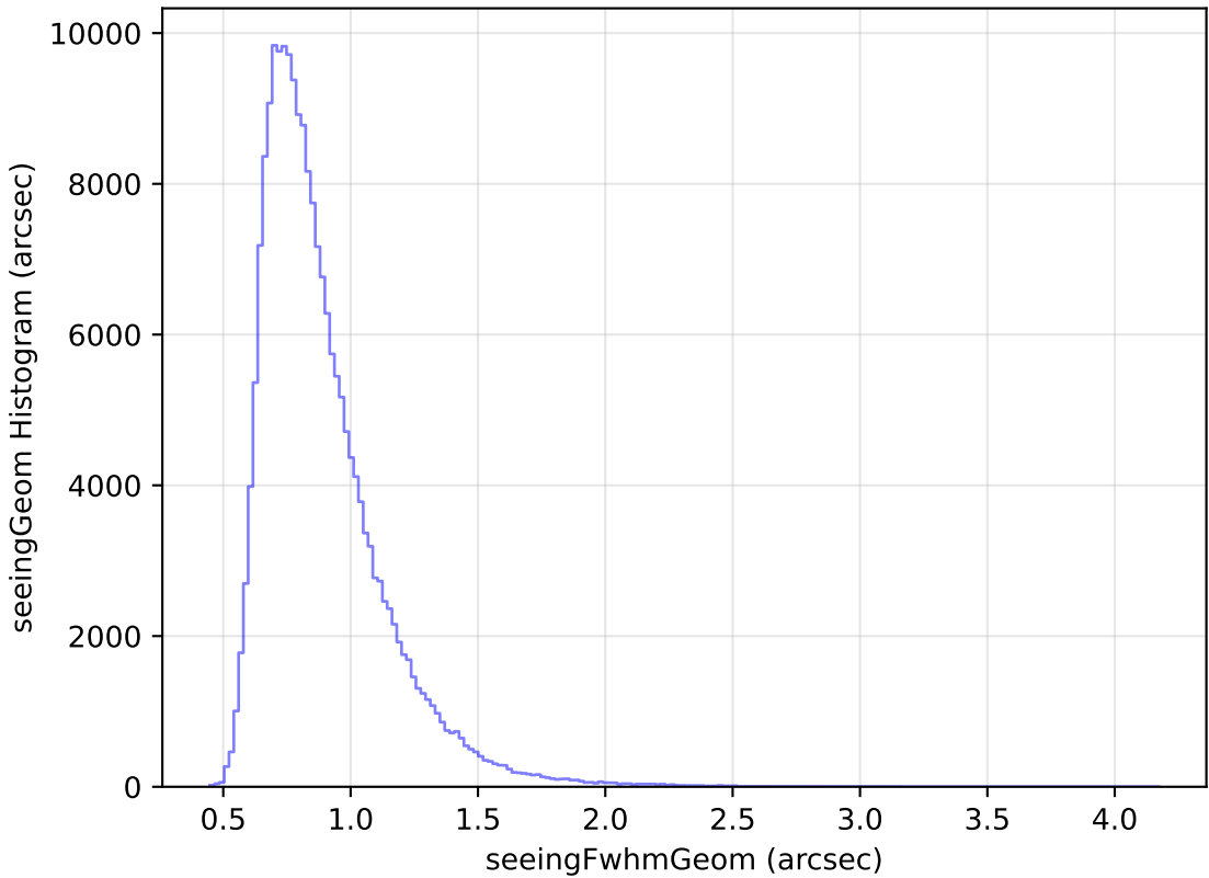
weather_cloudso31v3.4_10yrs Yr 1 all bands: seeingGeom Histogram
