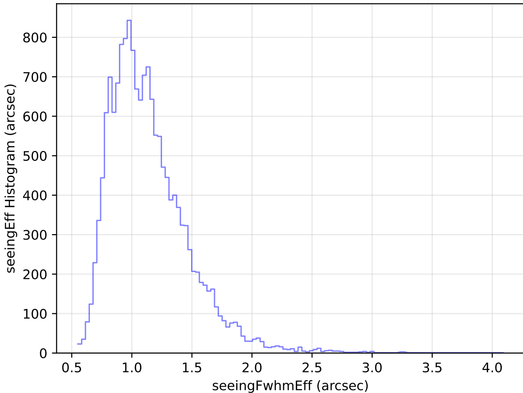
weather_cloudso31v3.4_10yrs Yr 1 u band: seeingEff Histogram
