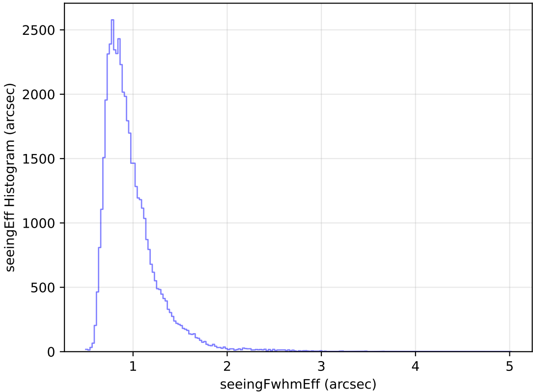
weather_cloudso31v3.4_10yrs Yr 1 i band: seeingEff Histogram
