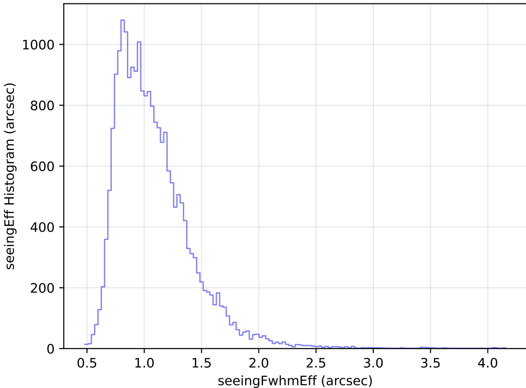
weather_cloudso31v3.4_10yrs Yr 1 g band: seeingEff Histogram
