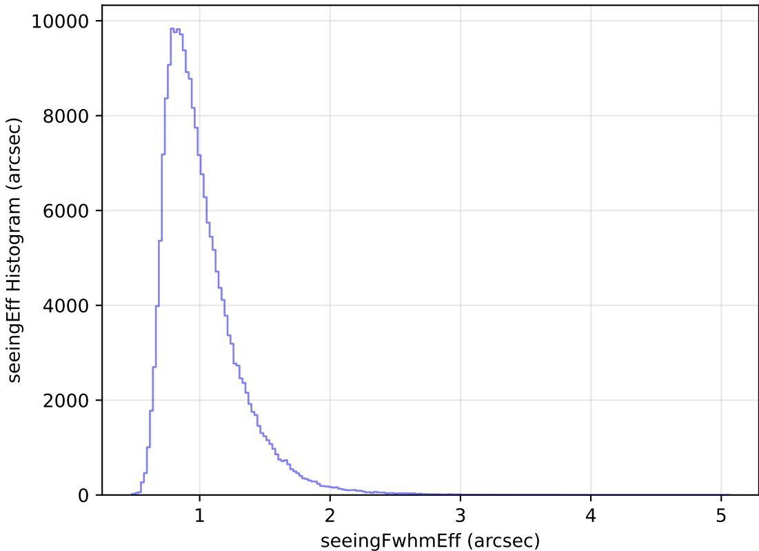
weather_cloudso31v3.4_10yrs Yr 1 all bands: seeingEff Histogram
