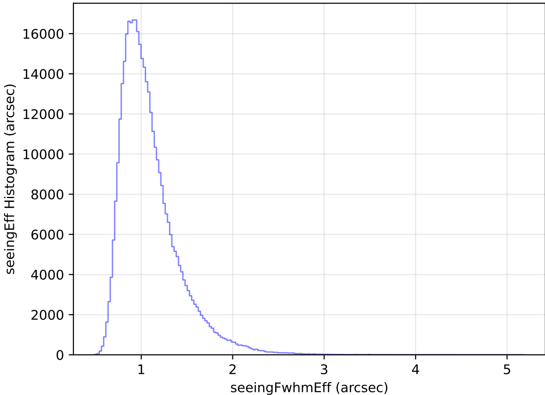
weather_cloudso31v3.4_10yrs WFD y band: seeingEff Histogram
