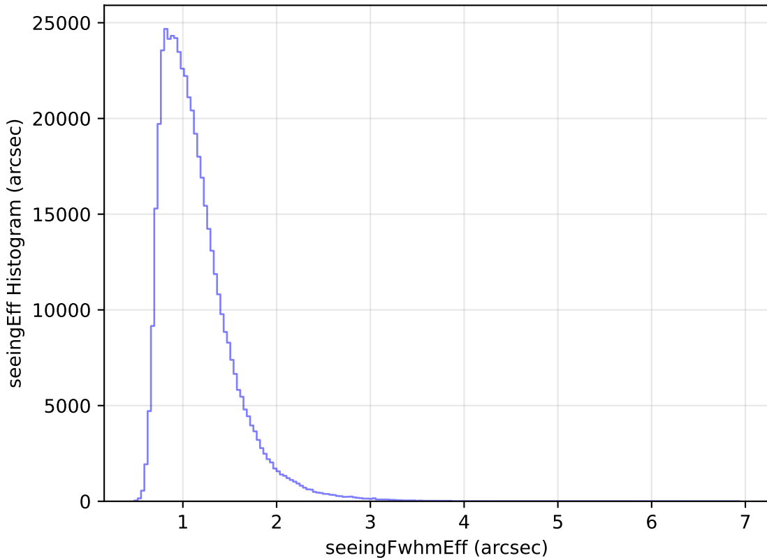
weather_cloudso31v3.4_10yrs WFD r band: seeingEff Histogram
