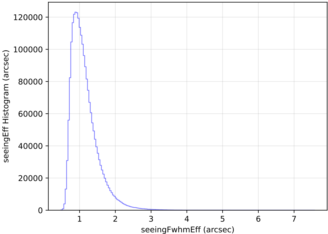
weather_cloudso31v3.4_10yrs WFD all bands: seeingEff Histogram
