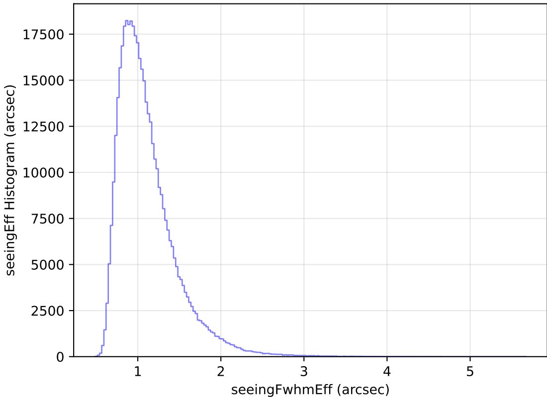
weather_cloudso31v3.4_10yrs All sky z band: seeingEff Histogram
